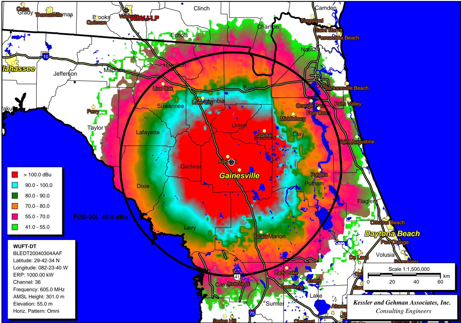
WUFT-DT Channel 36 (License) Longley-Rice Interference-Free Coverage Map
